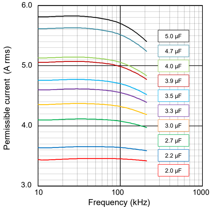
[ Permissible Current ]
