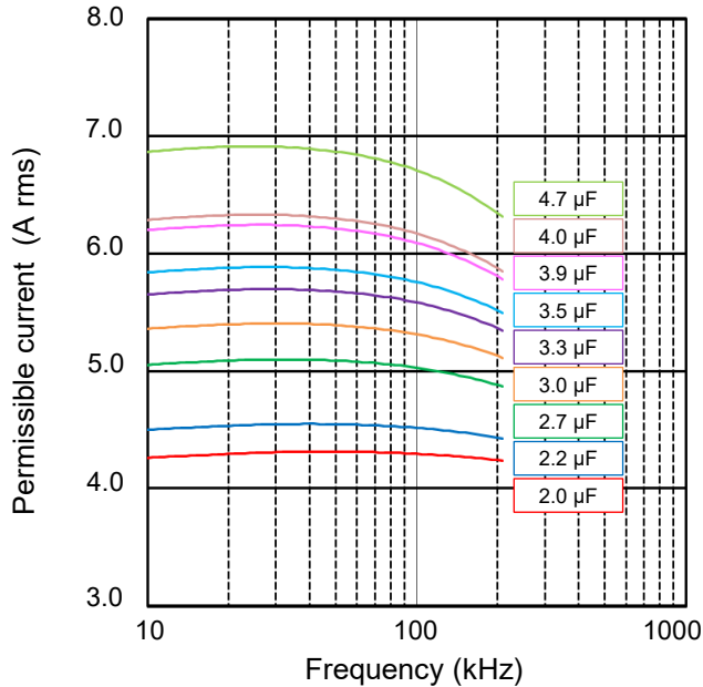
[ Permissible Current ]
