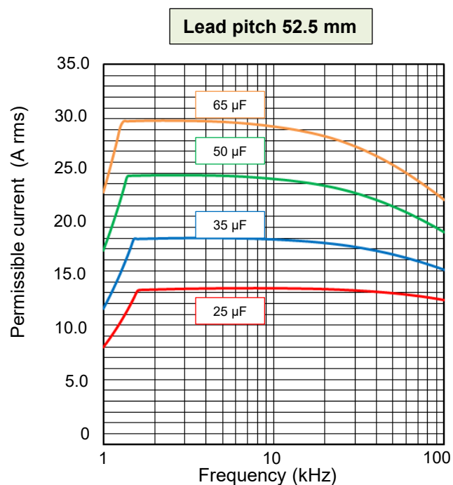
[ Permissible Current ]
