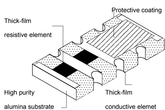
Fig.4. Chip resistor array (convex-type)
