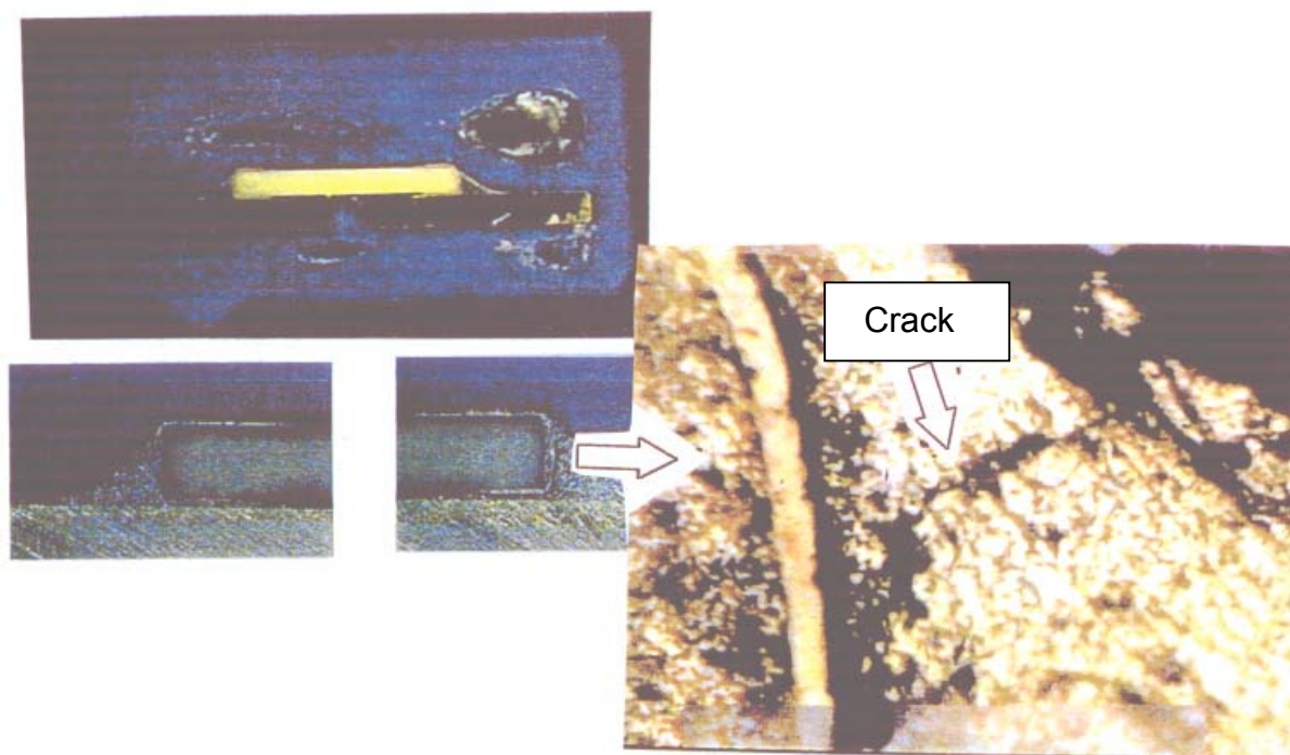
Fig.26. Disconnection by resin mold of chip resistors
